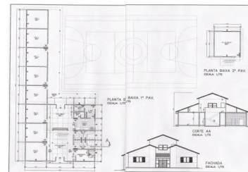
Architects blueprints of AmerinRio Cultural Center in Rio de Janeiro.
